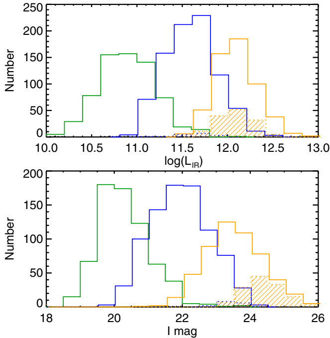
Figure 1. Distribution of Herschel -selected galaxies included in this study in L_{\text{IR}} and I -band magnitude. Green, blue, and orange indicate three redshift bins: 0.2 < z < 0.5 , 0.5 < z < 1.0 , and 1.0 < z < 1.5 . The shaded area illustrates the distribution of unclassifiable objects in each redshift bin. Note that although the histograms for different redshift bins have exactly the same location, the distributions are offset slightly from each other in the plot for clarity.
