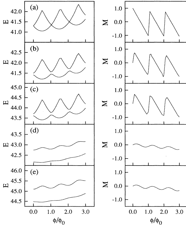
FIG. 2. The lowest two energy values and magnetization vs \Phi/\Phi_0 for a four-electron system at \alpha = 20 . (a) Noninteracting and impurity-free, (b) noninteracting, but with impurity potential ( V_0 = 1.0, d = 0.2 ), (c) interaction and impurity included ( V_0 = 1.0, d = 0.2 ), (d) noninteracting, but with impurity included ( V_0 = 4.0, d = 0.5 ), and (e) interaction and impurity included ( V_0 = 4.0, d = 0.5 ).
