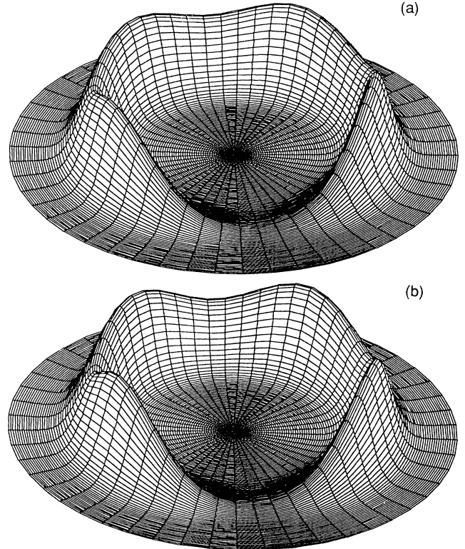
FIG. 4. The charge density for \alpha = 20, V_0 = 4.0, d = 0.5 , with (a) noninteracting but impurity included and (b) impurity and interactions included.
