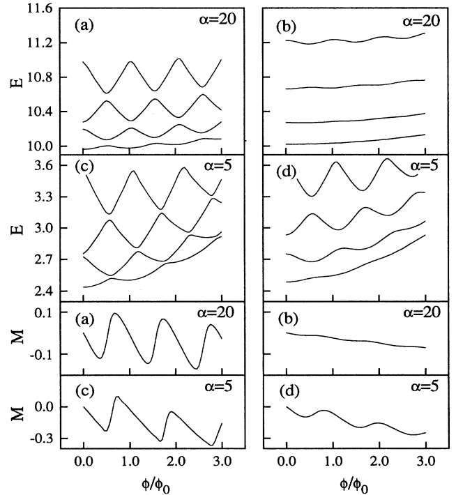
FIG. 1. Single-electron energy spectrum and magnetization (in units of energy defined in the text) vs \Phi/\Phi_0 for (a) \alpha = 20 , V_0 = 1.0 , d = 0.2 ; (b) \alpha = 20 , V_0 = 4.0 , d = 0.5 ; (c) \alpha = 5 , V_0 = 0.5 , d = 0.2 ; and (d) \alpha = 5 , V_0 = 1.0 , d = 0.5 .
