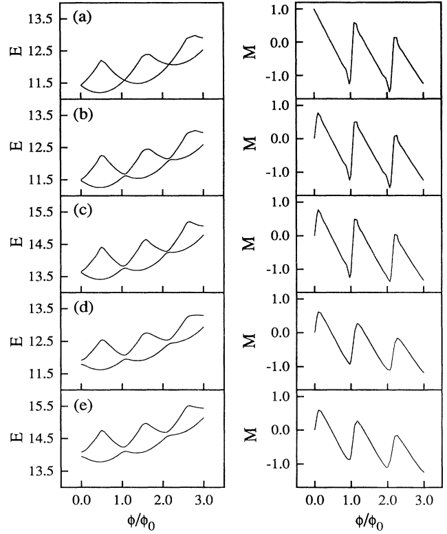
FIG. 3. Same as in Fig. 2, but for \alpha = 5 , and V_0 = 0.5, d = 0.2 [(b) and (c)] and V_0 = 1.0, d = 0.5 [(d) and (e)].
