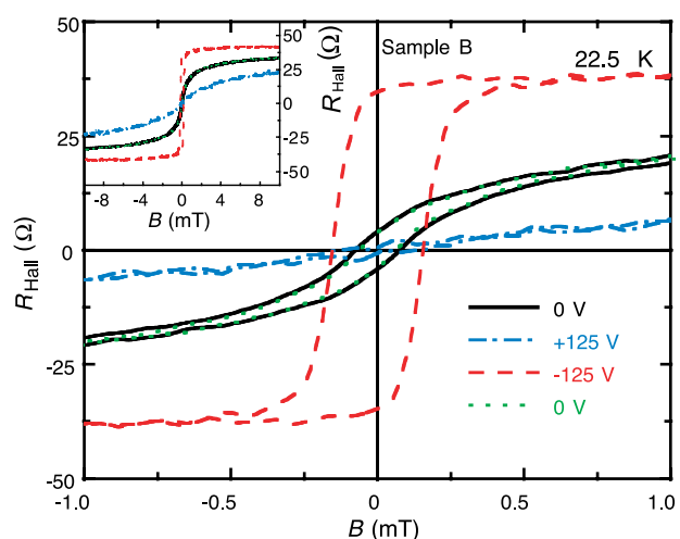
Fig. 5. Field effect control of hole-induced ferromagnetism in magnetic semiconductor (In,Mn)As field-effect transistors. Shown is magnetic field dependence of the sheet Hall resistance R_{Hall} , which is proportional to the magnetization of the magnetic semiconductor layer, as a function of the applied gate voltage V_G . R_{Hall} is used to measure the small magnetization of the channel. V_G controls the hole concentration in the magnetic semiconductor channel. Application of V_G = 0 , +125, and -125 V results in qualitatively different field dependence of R_{Hall} measured at 22.5 K. When holes are partially depleted from the channel ( V_G = +125 V), a paramagnetic response is observed (blue dash-dotted line), whereas a clear hysteresis at low fields ( < 0.7 mT) appears as holes are accumulated in the channel ( V_G = -125 V, red dashed line). Two R_{Hall} curves measured at V_G = 0 V before and after application of \pm 125 V (black solid line and green dotted line, respectively) are virtually identical, showing that the control of ferromagnetism can be done isothermally and reversibly. (Inset) The same curves shown at higher magnetic fields. [Adapted from (23)]
